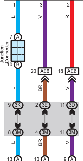
A56(A), E40(B) Junction Connector
